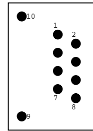
CONECTOR RJ45 VISTA SUPERIOR
