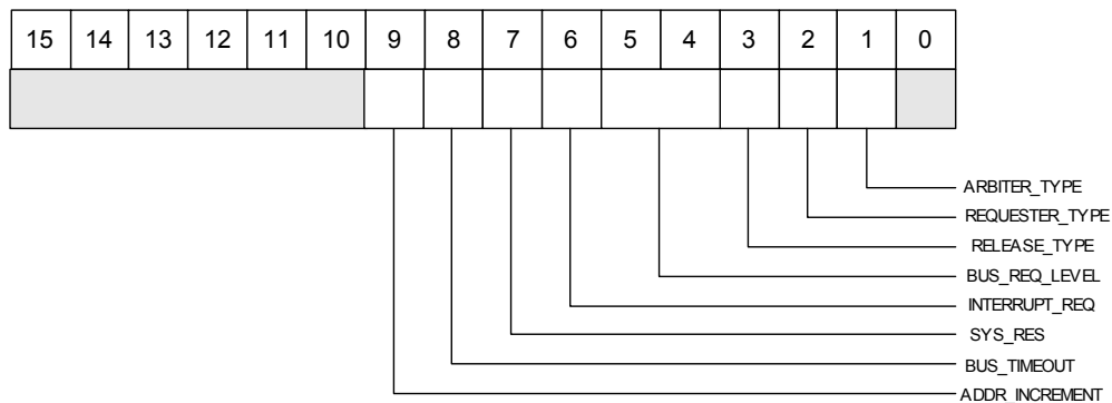
Fig. 2.5: Control Register
