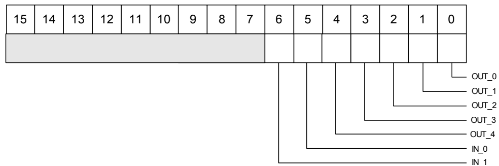
Fig. 2.15: LED Polarity set register
