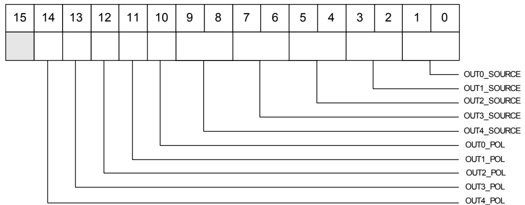
Fig. 2.13: Output Multiplexer Set register
