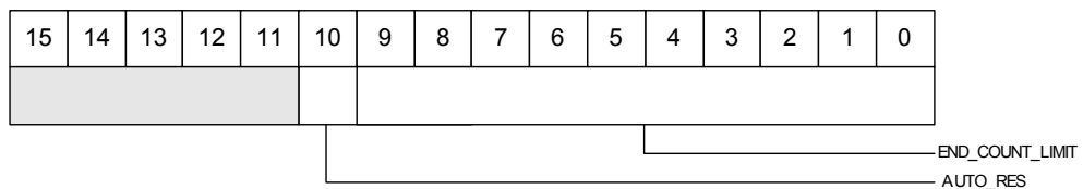
Fig. 2.21: Scaler 0 register
