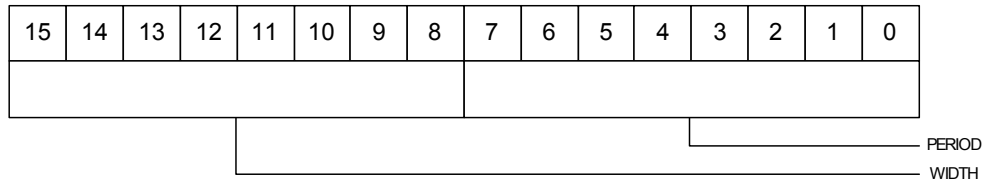
Fig. 2.19: Pulser B 0 register
