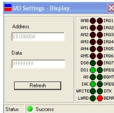
Fig. 4.8: The I/O Setting Menu – Display
