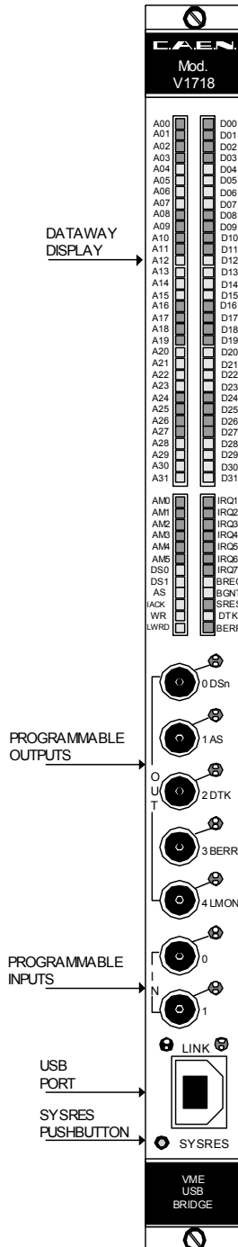
Fig. 3.1: Mod. V1718 front panel
