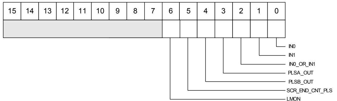
Fig. 2.8: Input register
