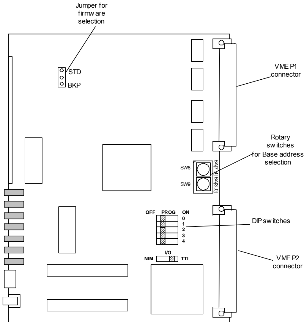
Fig. 3.3: Component Location
