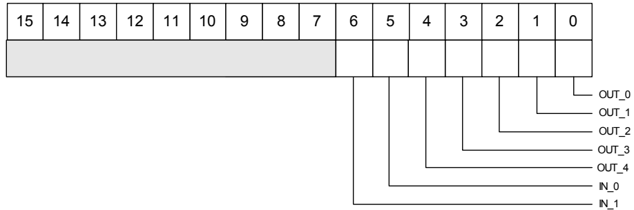
Fig. 2.16: LED polarity clear register
