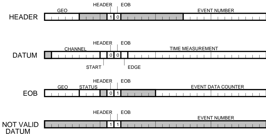
Fig. 3.4: Mod. V767 Output Buffer Data Structure
