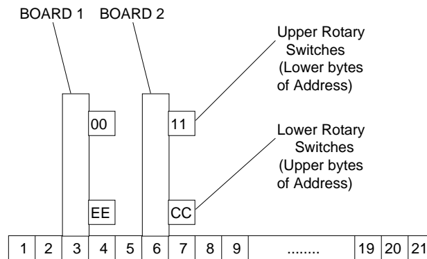
Fig. 3.1: Base/GEO Addressing Example 1
