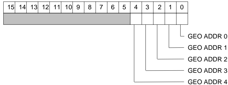
Fig. 3.5: GEO Address Register
