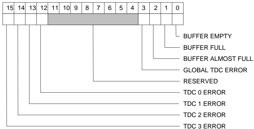
Fig. 3.15: Status Register 2
