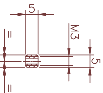
DETALLE ROSCA TALADROS
